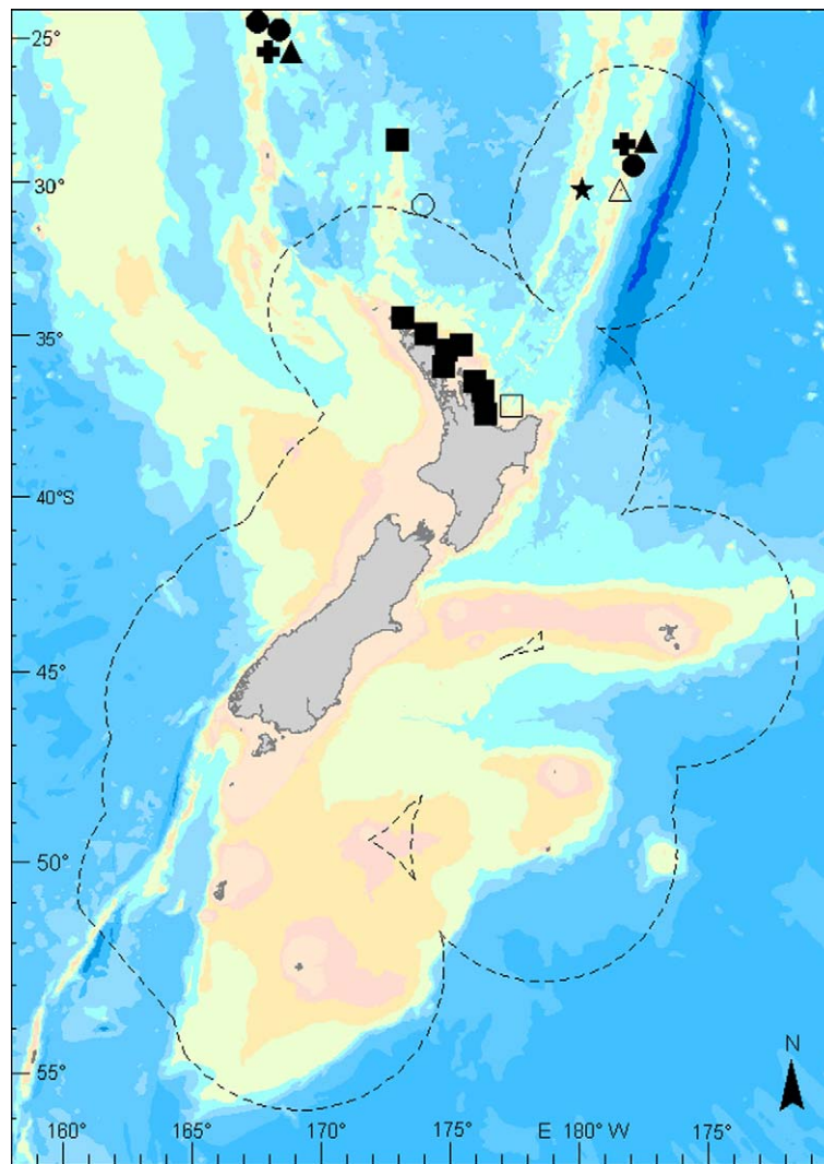
FIGURE 3. Distribution map of ogcocephalid species found in New Zealand waters. Square = Halieutaea stellata ; star = Halieutopsis bathyoreos ; triangle = Malthopsis asperata ; cross = Malthopsis mitrigeria ; and circle = Malthopsis parva . One dot may represent more than one capture. Open dots indicate the holotype localities, including the holotype of H. maoria (open square).
