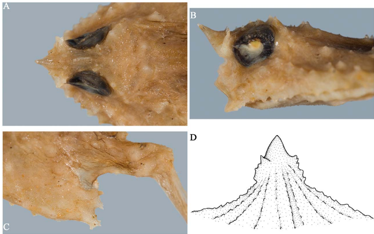
FIGURE 2. Malthopsis asperata sp. nov., from the holotype. A. closed view of dorsal head. B. closed view of lateral head. C. closed view of left subopercular region. D. lateral view of dorsal buckler, about 2 mm width, illustrated by M. Freebone. A–C. photo by C. Struthers.
