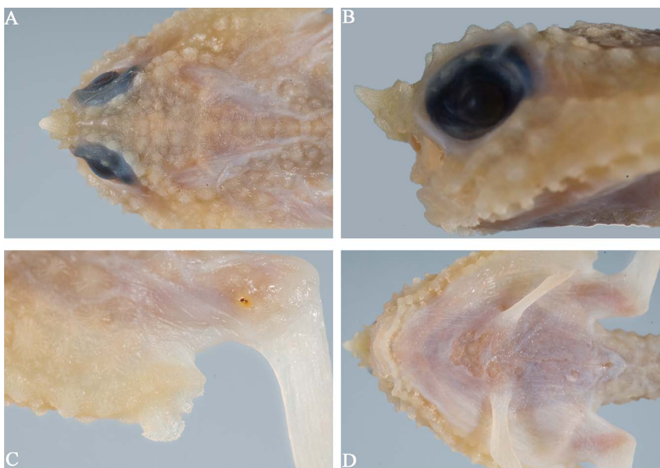
FIGURE 5. Malthopsis parva sp. nov. , holotype. A. closed view of dorsal head. B. closed view of lateral head. C. closed view of left subopercular region. D. ventral view of disc showing the naked area and some flattened bucklers at pelvic fin base area. Photo by C. Struthers.
