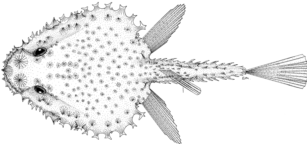
FIGURE 8. Halieutopsis bathyoreos Bradbury, 1988, NMNZ P.017314, 32.0 mm SL, dorsal view, illustrated E. Mackay.
