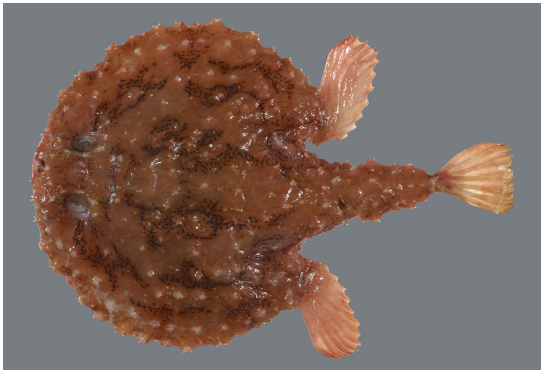
FIGURE 7. Halieutaea stellata (Vahl, 1797), NMNZ P.0, 198 mm SL, fresh, dorsal view, photo by C. Struthers.
