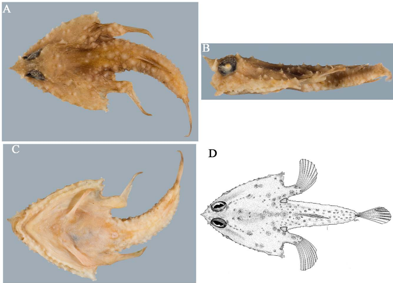
FIGURE 1. Malthopsis asperata sp. nov., holotype, NMNZ P.035177, 65.4 mm SL. A. dorsal view. B. lateral view. C. ventral view. D. drawing of dorsal view, illustrated by E. Mackay. A–C. photo by C. Struthers.
